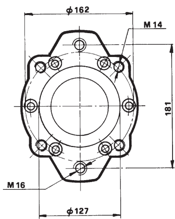
SAE C 2-4 holes 30431 - 30432
